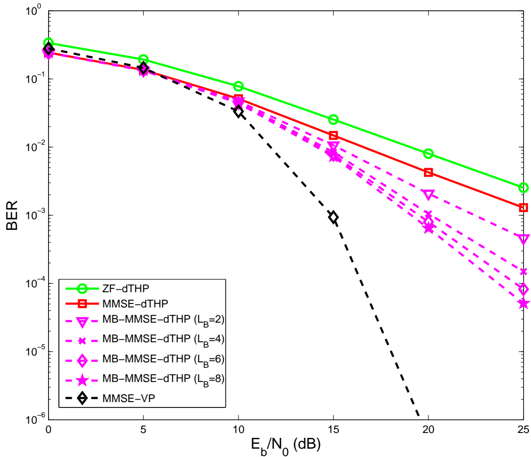
Figure 5.7: BER performance of c THP, QPSK.
