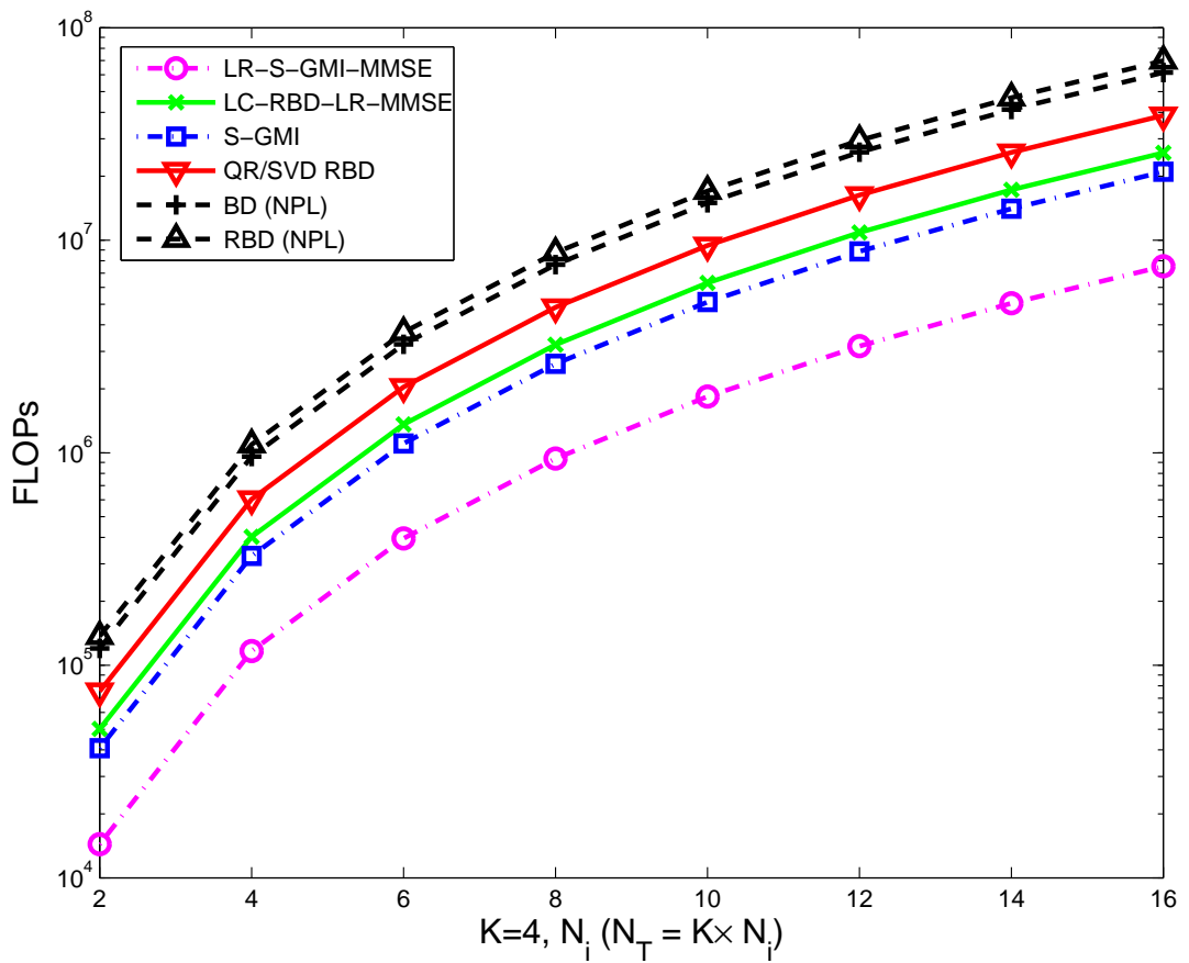
Figure 4.4: Computational Complexity - II Fixed K
