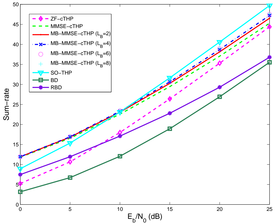
Figure 5.9: Sum-rate performance of dTHP.
