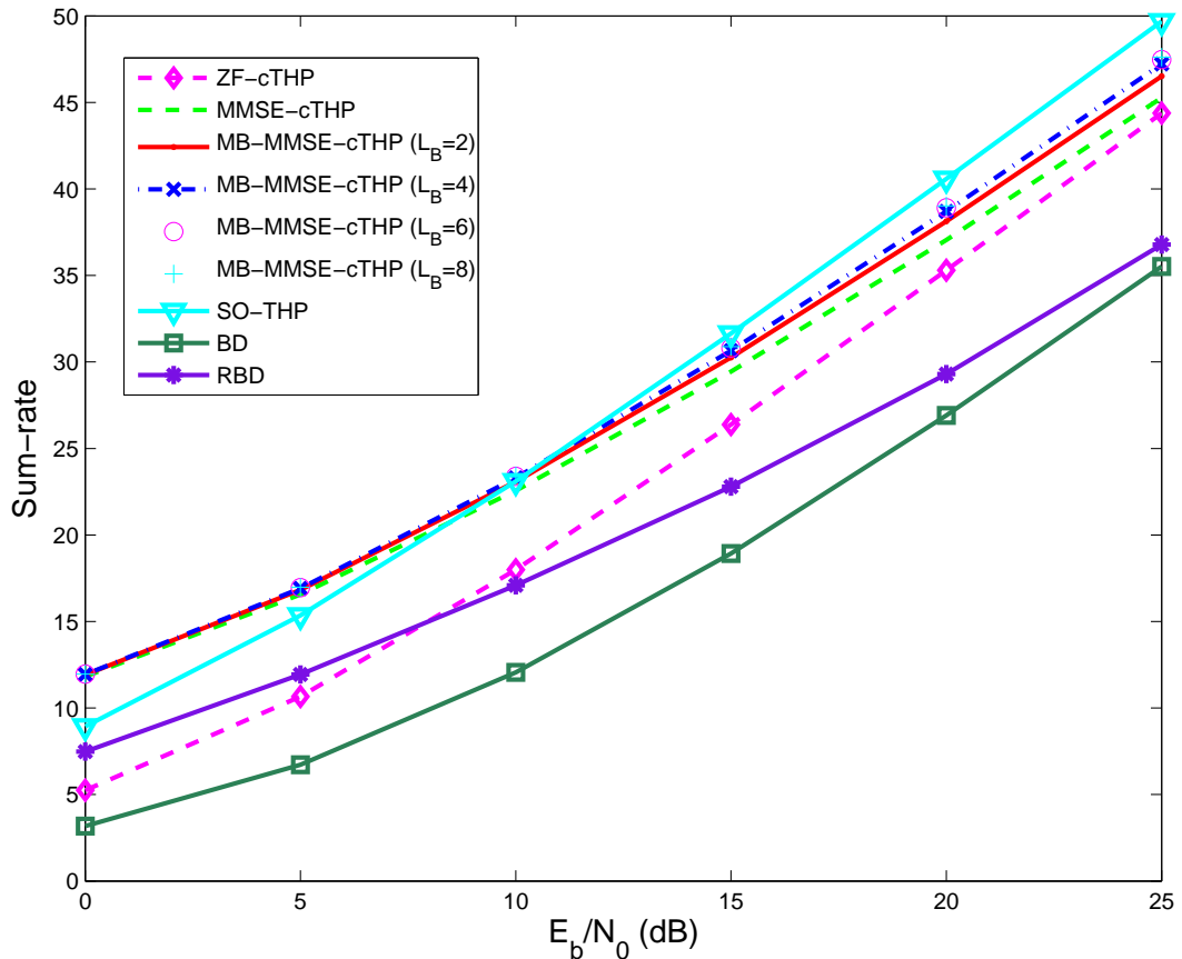
Figure 5.8: Sum-rate performance of cTHP.
