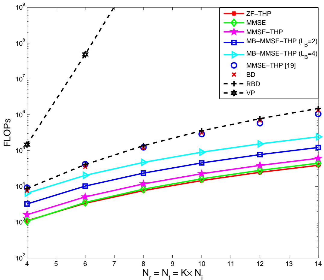
Figure 5.2: Complexity Analysis
