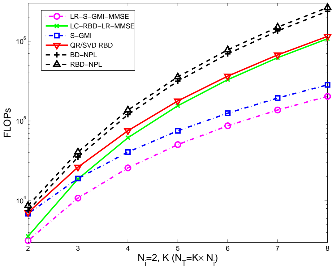
Figure 4.3: Computational Complexity - I Fixed N_k
